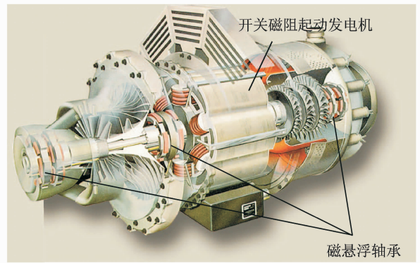
图 11 基于内装式开关磁阻发电机系统的集成动力装置 Fig. 11 Integrated power unit with internal switched reluctance starter/generator system
