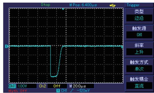
(b) Triode collector pulse signal
